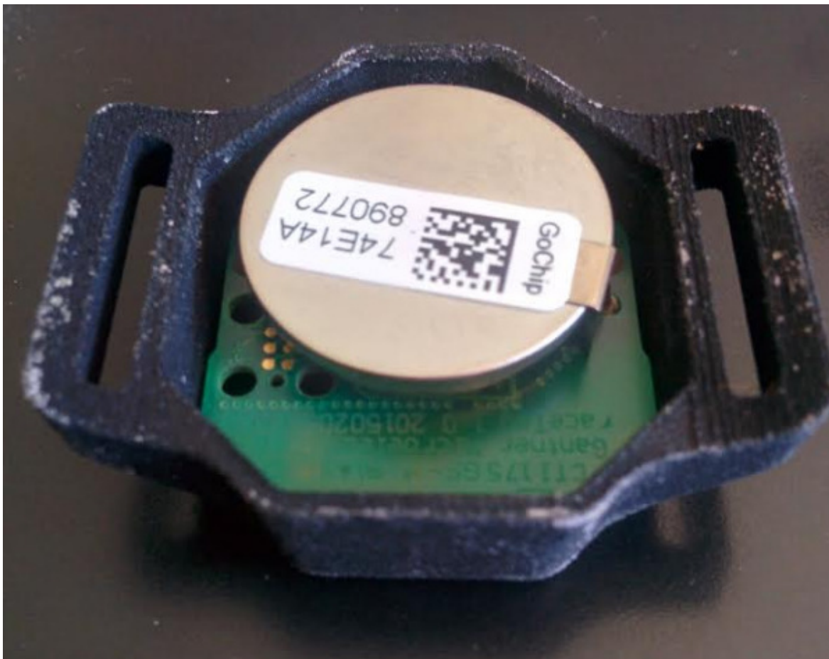
Figure 4: After urethane potting
