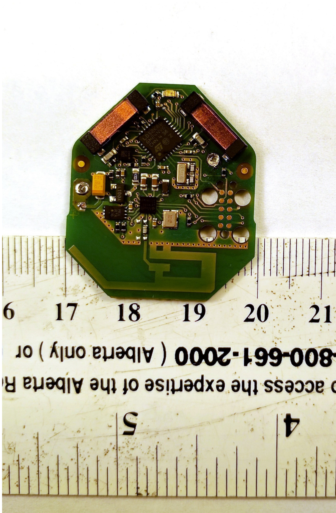
Figure 1: PC Board component side
