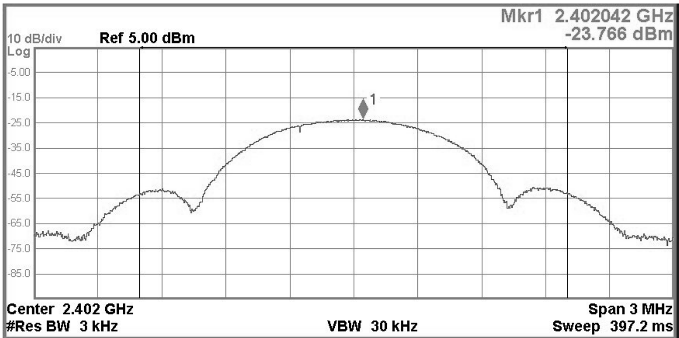
Screen Capture from the spectrum analyzer: 2402 MHz:
