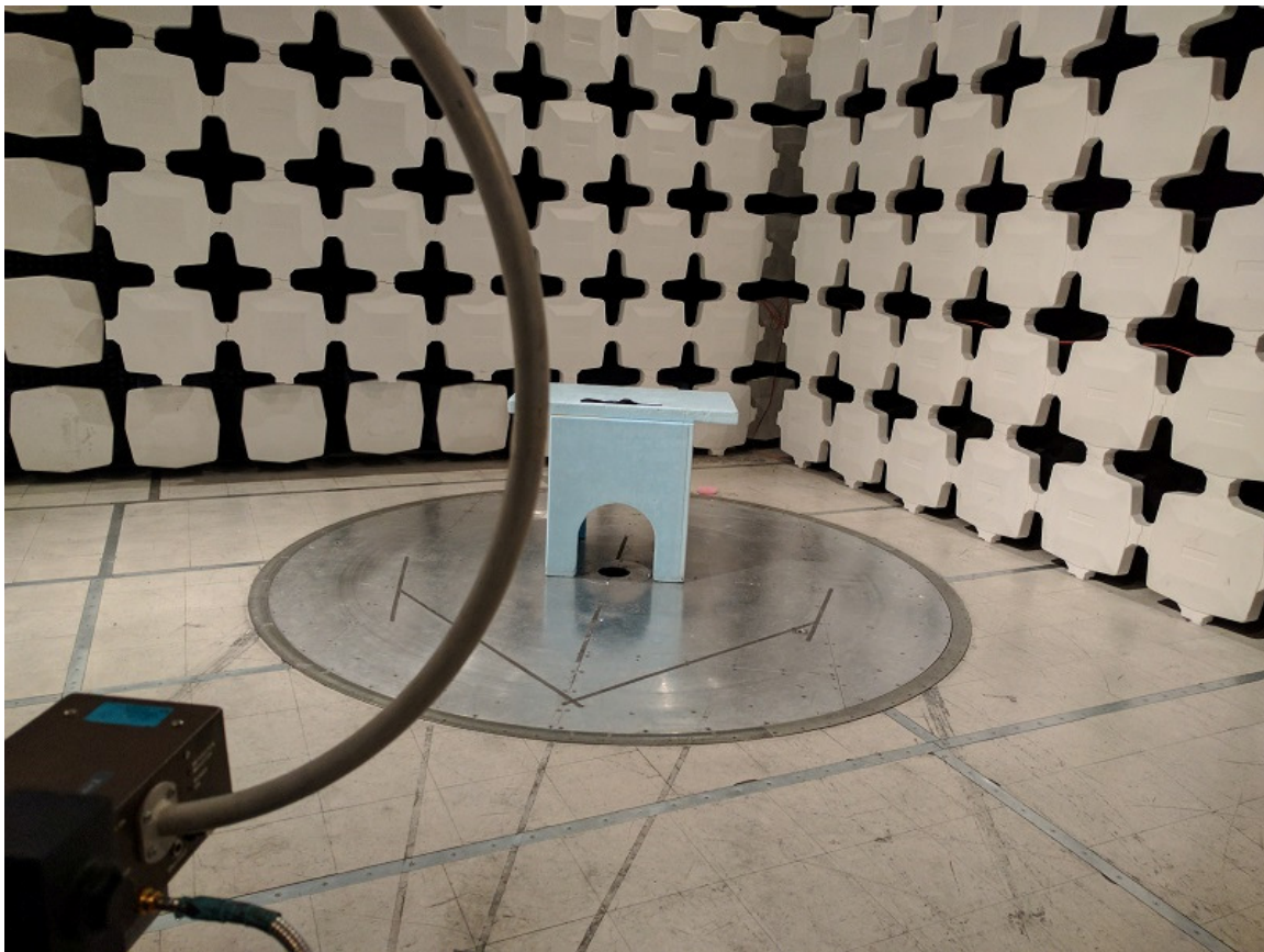
Figure 2 – Radiated Emissions, 9 kHz to 30 MHz:
