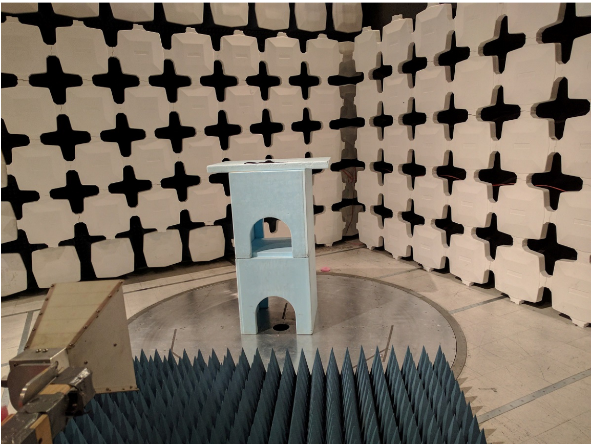
Figure 4 – Radiated Emissions, 1 GHz to 12 GHz:
