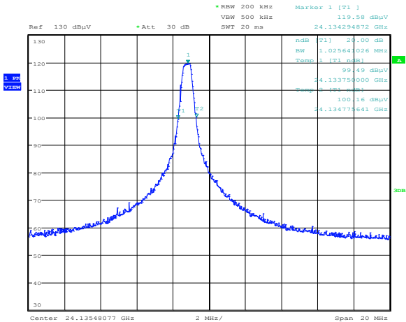
Figure 8.1-1: 20 dB bandwidth
