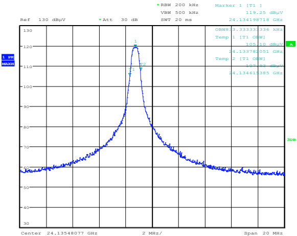
Figure 8.1-2: 99% occupied bandwidth
