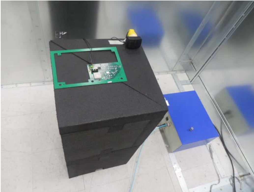
AC Mains Emissions
