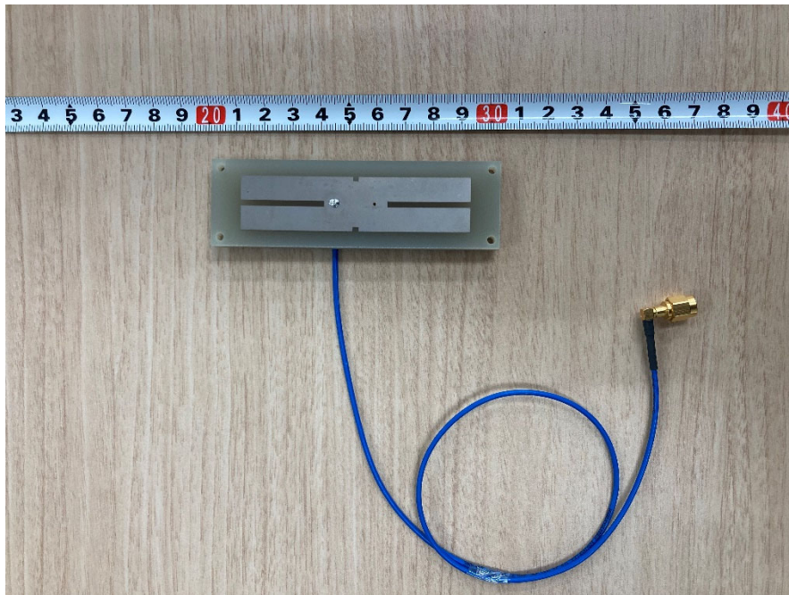
Antenna 1
