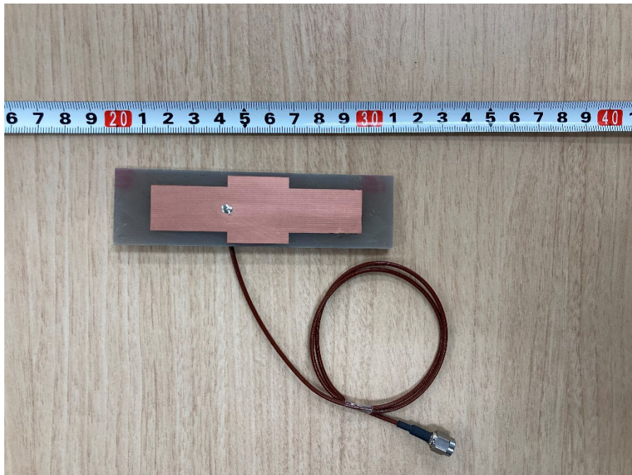
Antenna 2
