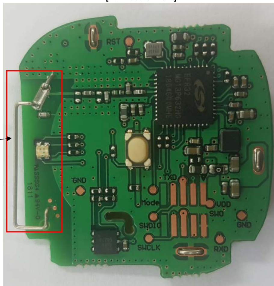
[Main board Front]
