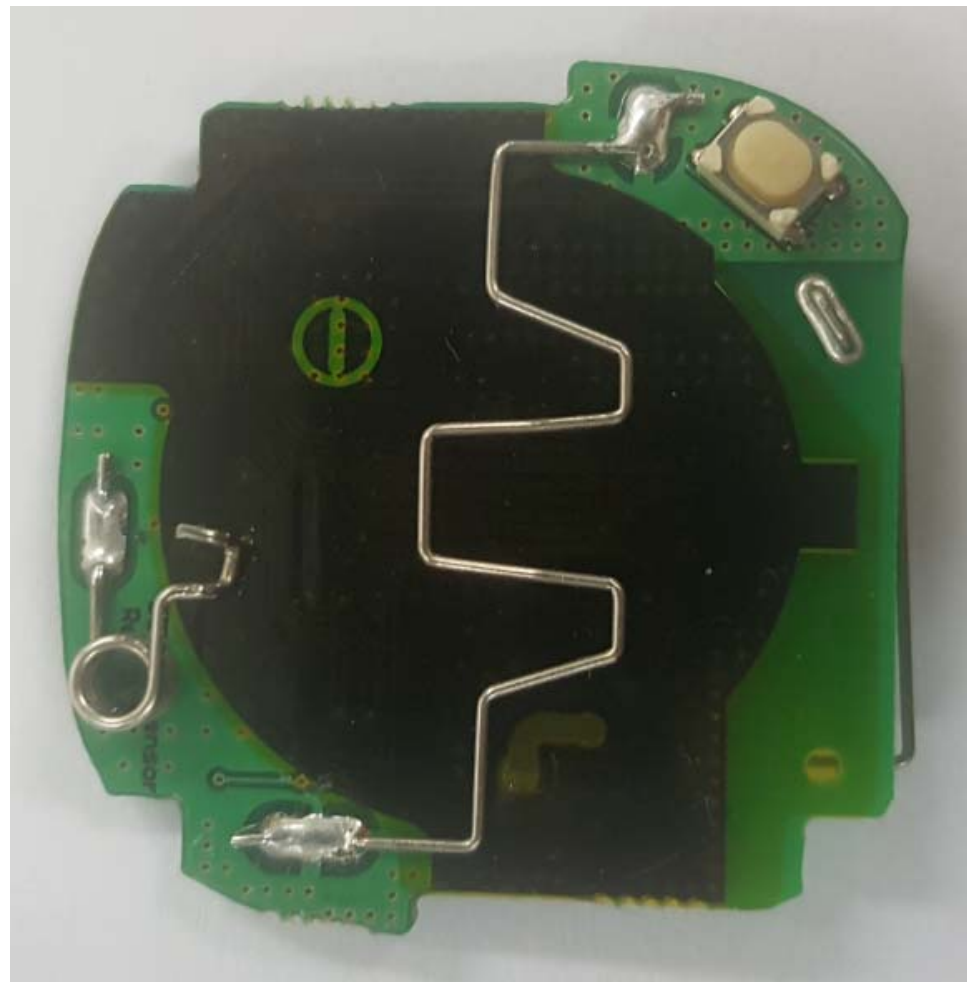
[Main board Rear]
