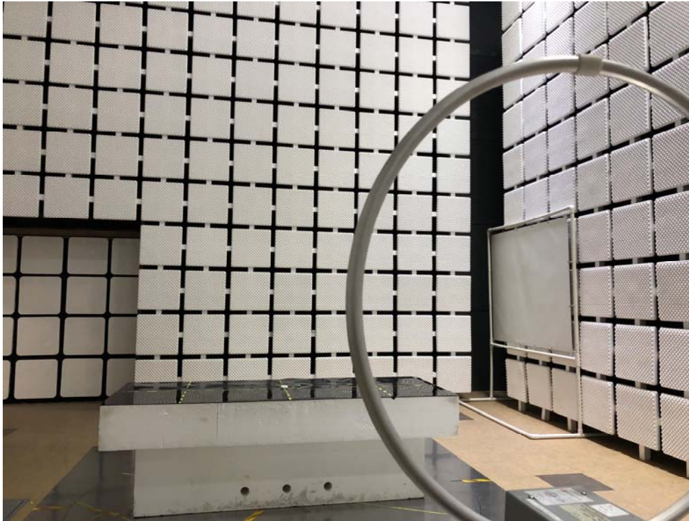
Radiated RF measurement (Below 30 MHz ~ 1 GHz)
