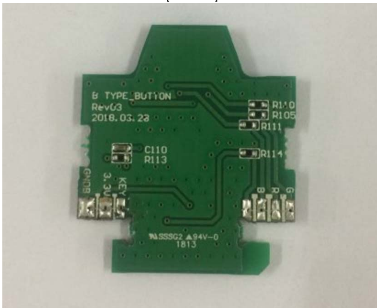
[Button Rear]
