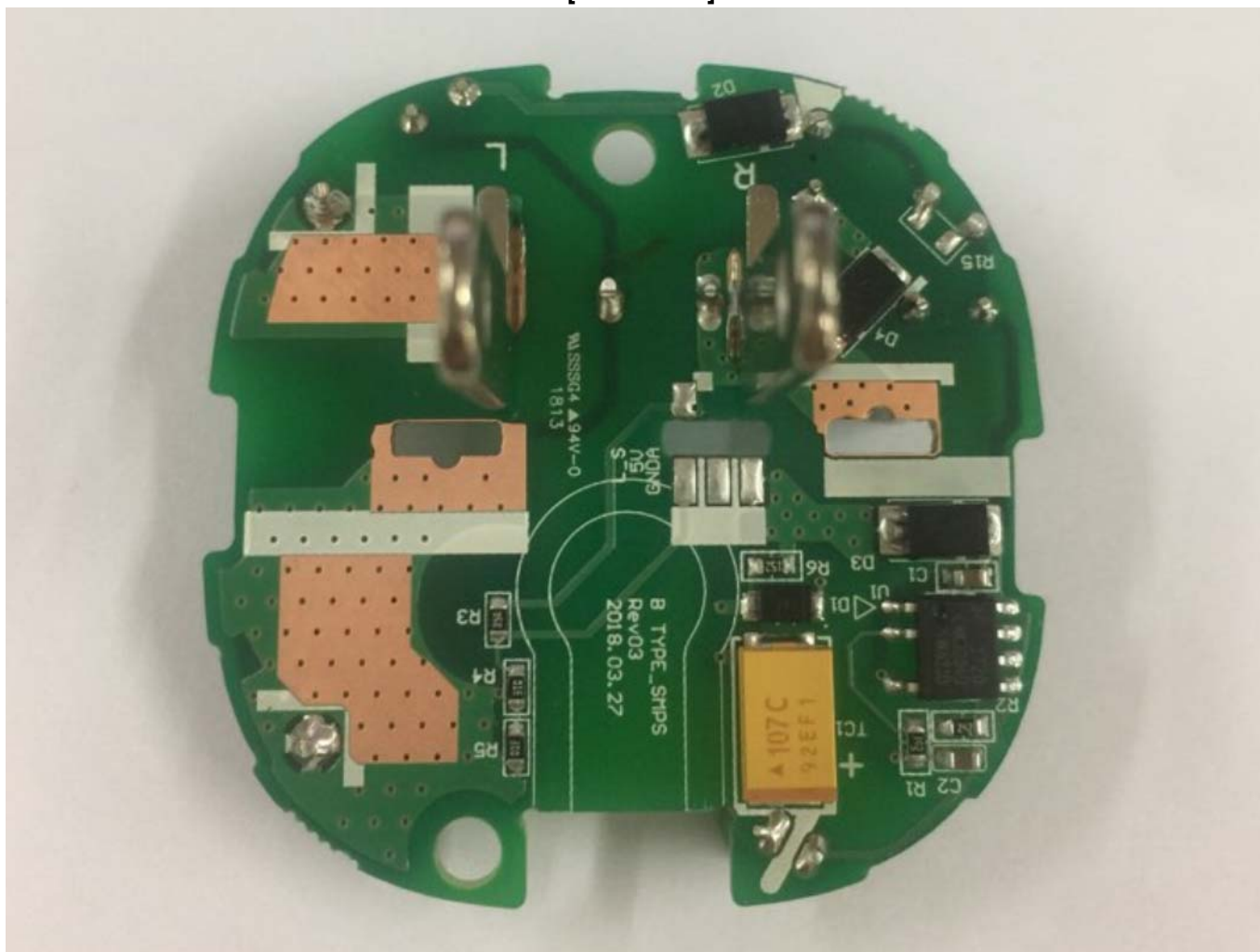
[SMPS Rear]
