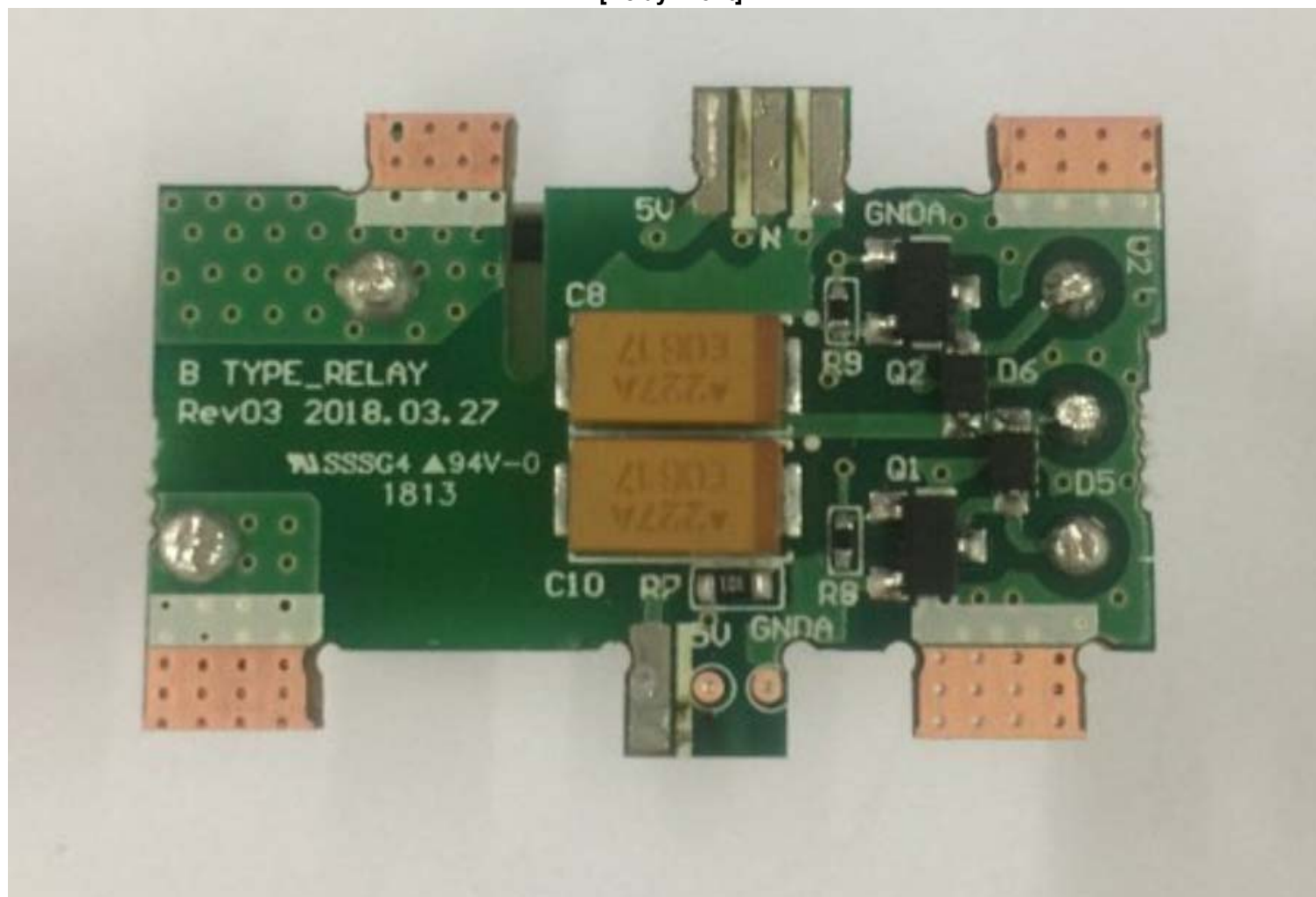
[Relay Front]
