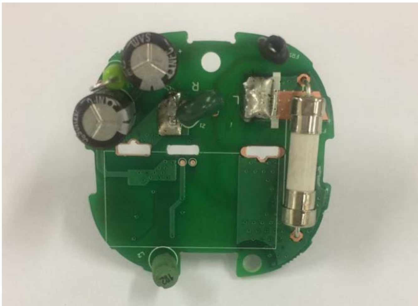
[SMPS Front]
