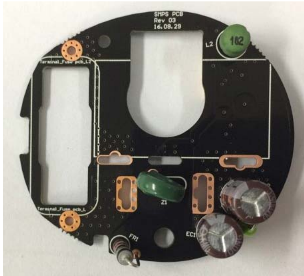
[SMPS board Front]
