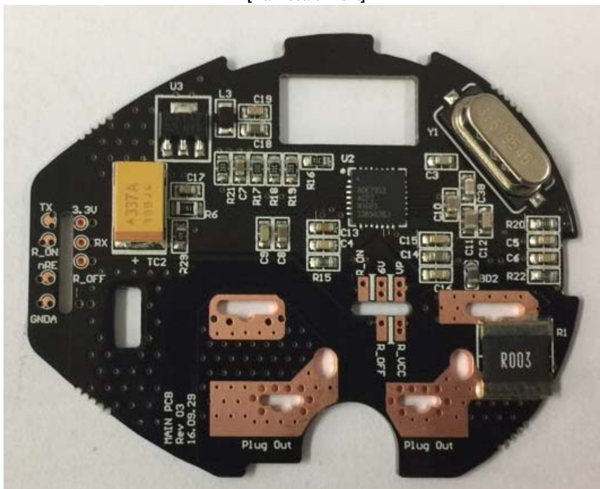
[Main board Front]
