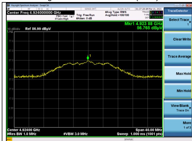
High channel 2 nd harmonic (Peak)
