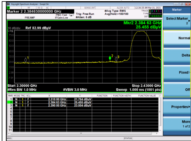
Low channel band edge (Peak)
