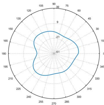
Total_Polar_E1_2.45GHz
