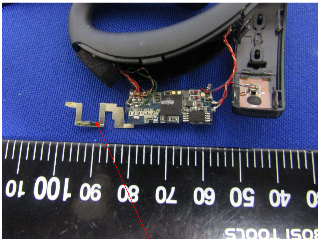
BT Antenna
