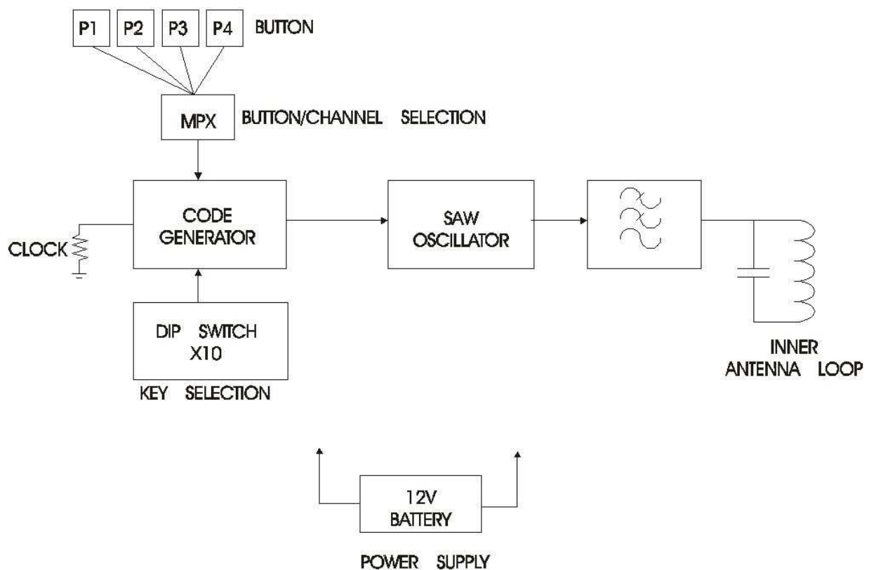
Figure 1 Block Diagram
