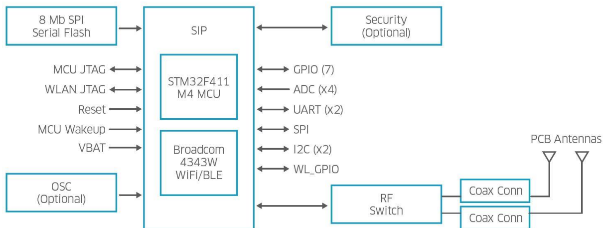
Figure 1 – AES-BCM4343W-M1-G Module Block Diagram
