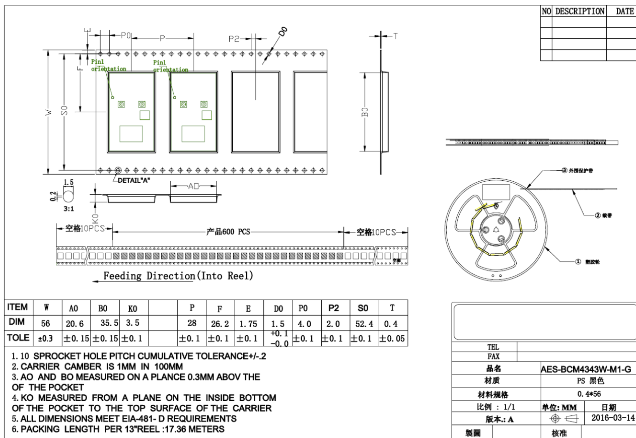
Figure 8 – Tape Dimensions
