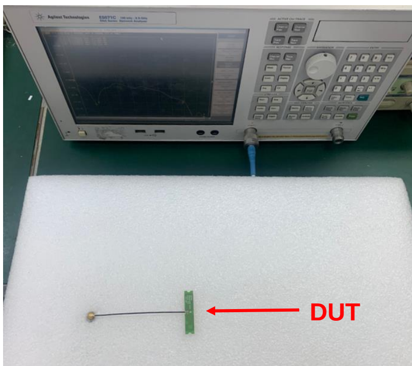
FIGURE4.1.1 ANTENNA IN FREE SPACE WITH VNA AGILENT E5071C
