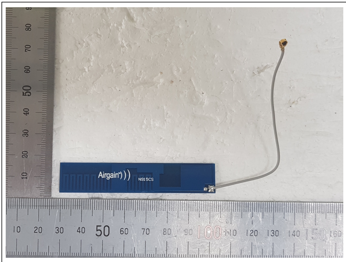
<915 MHz Antenna>
