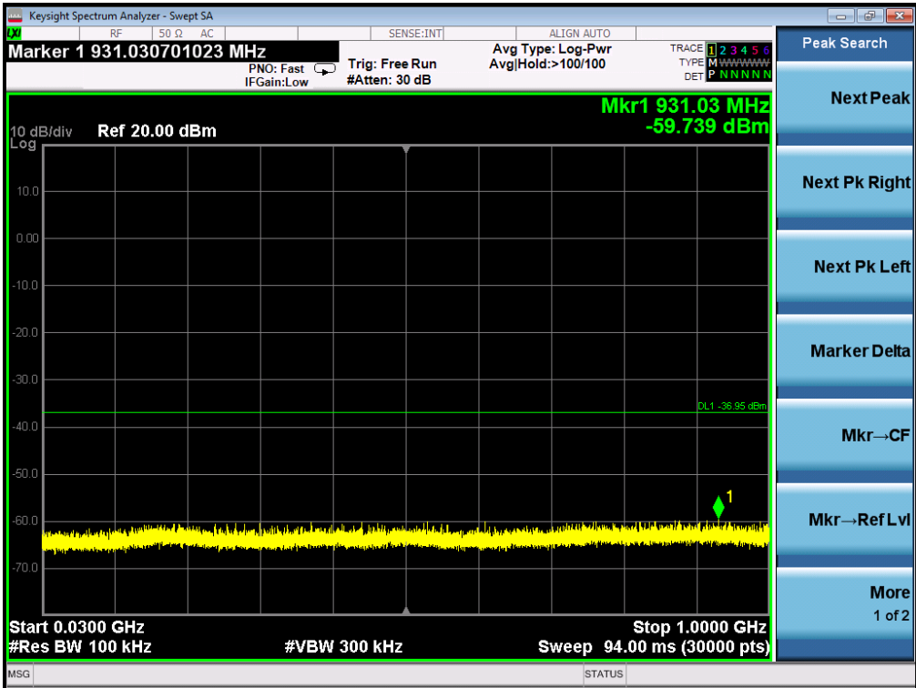
TEST PLOT OF OUT OF BAND EMISSIONS THE WORST CASE OF 802.11g FOR MODULATION IN MIDDLE CHANNEL
