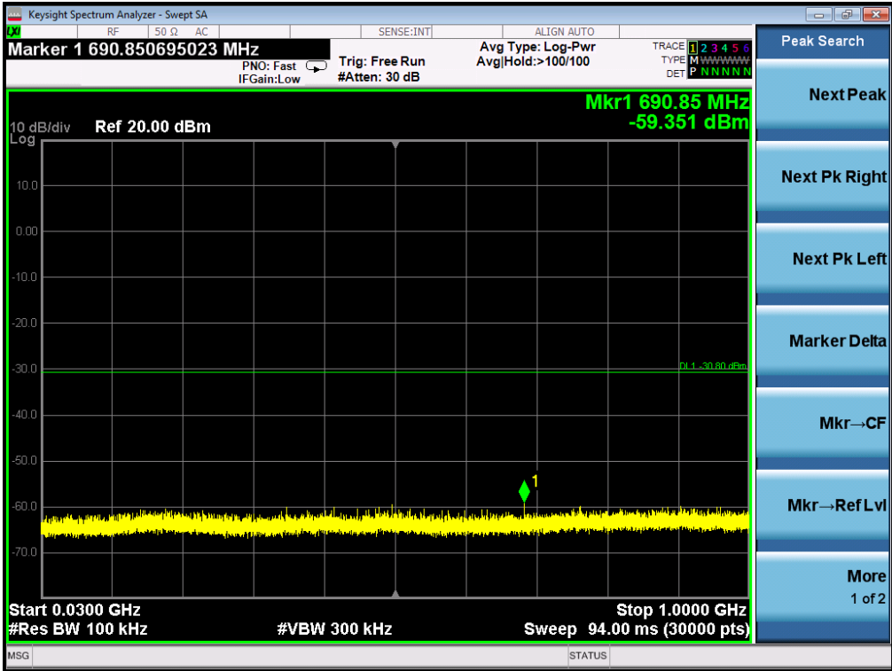
TEST PLOT OF OUT OF BAND EMISSIONS THE WORST CASE OF 802.11b FOR MODULATION IN HIGH CHANNEL
