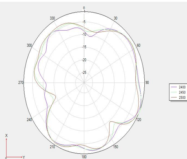
Theta 90 2D
