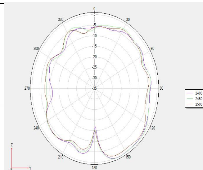
Phi 90 2D
