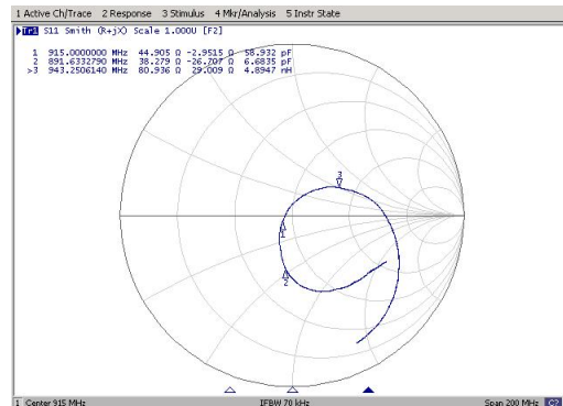
Smith Chart
