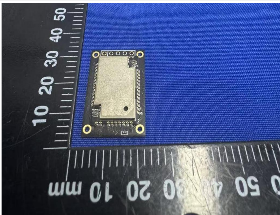
RIGHT VIEW OF EUT RAK3312
