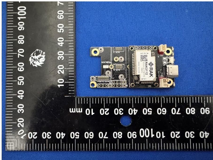
FRONT VIEW OF EUT WITH ACCESSORY POWER SUPPLY BOARD
