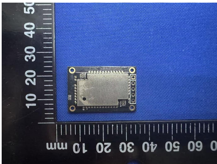
EUT TOP VIEW RAK3312
