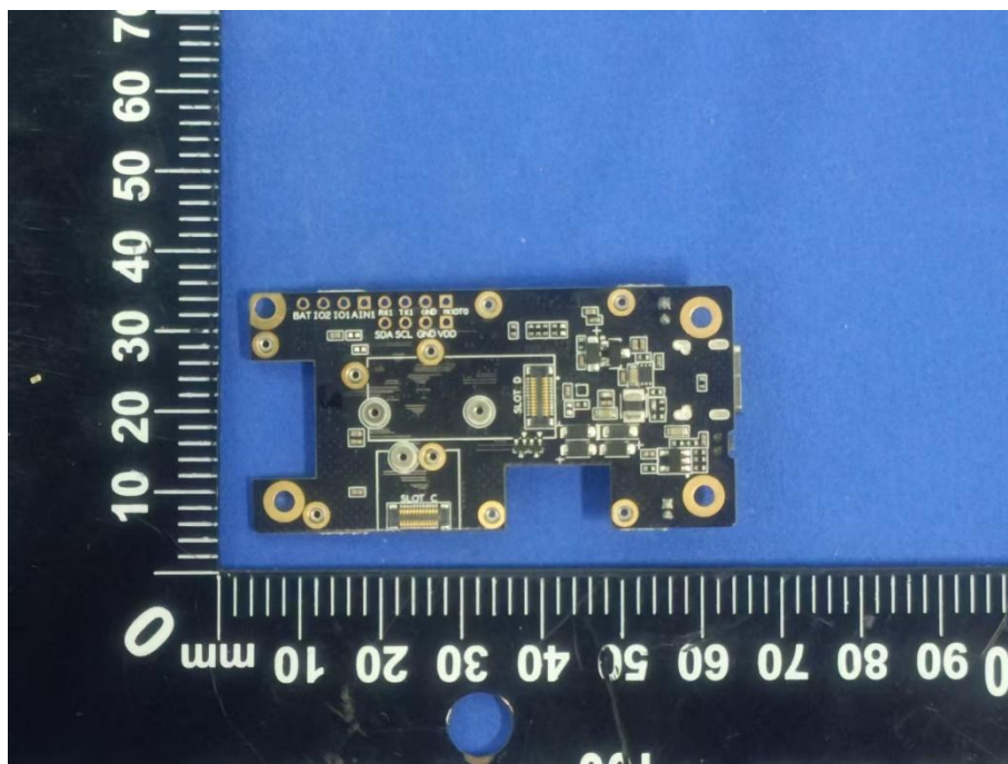
SECONDARY BOARD 1 REAR VIEW (WITH ACCESSORY POWER SUPPLY BOARD)
