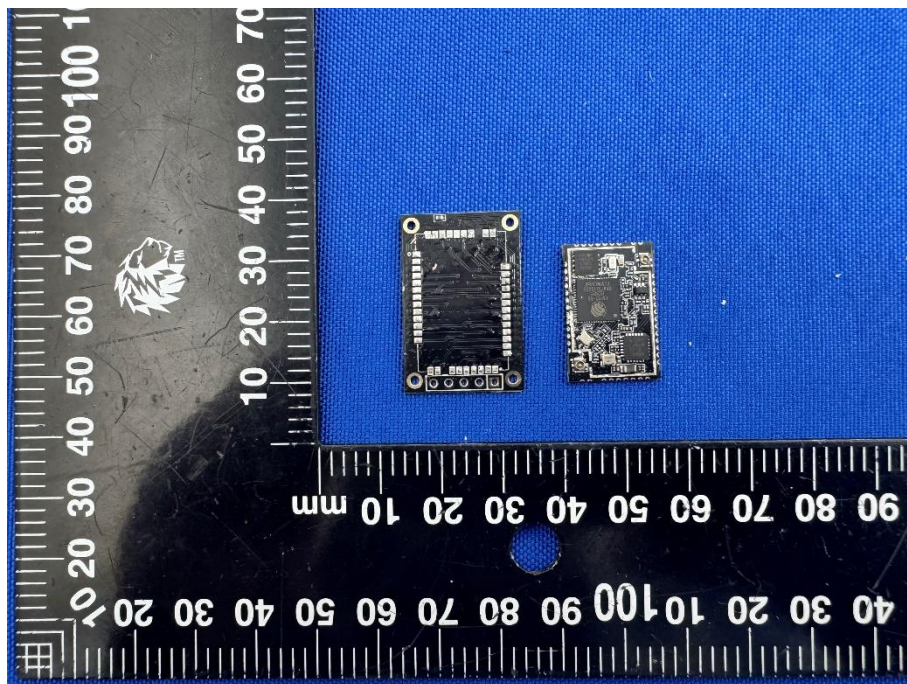
EUT TOP VIEW RAK3312 (WITHOUT SHIELDING)
