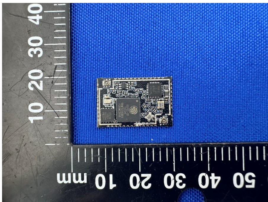
EUT TOP VIEW RAK3112 (WITHOUT SHIELDING)
