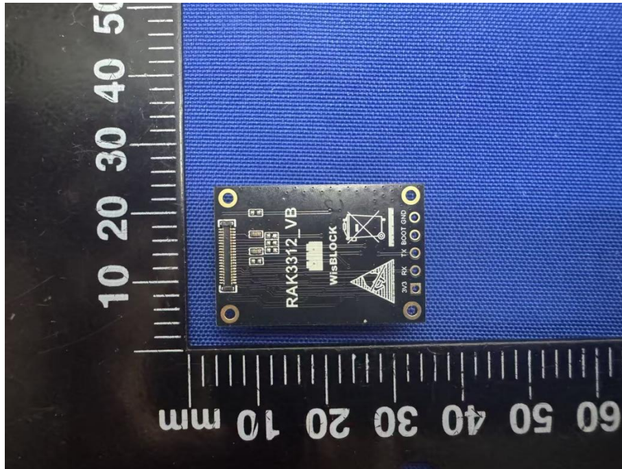
EUT REAR VIEW RAK3312
