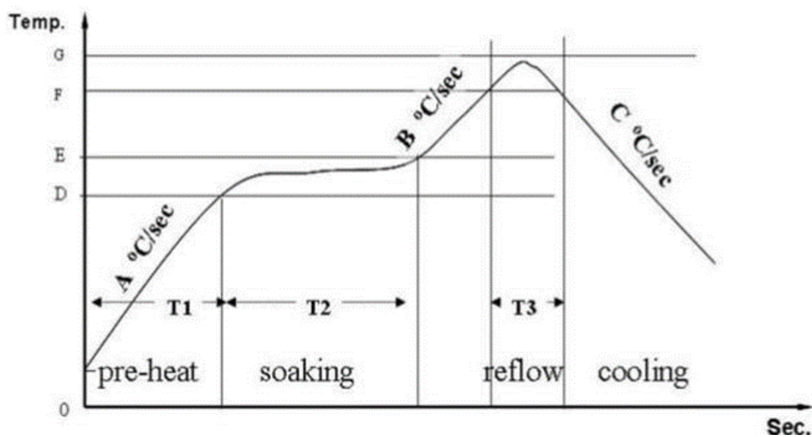
Figure 5:Reflow Profile for RAK3112
