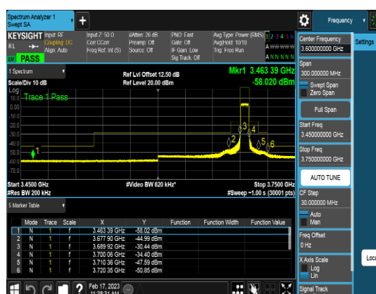
Port2_10M_3694.98MHz_TM3.1_CHH_CSEpart9 6
