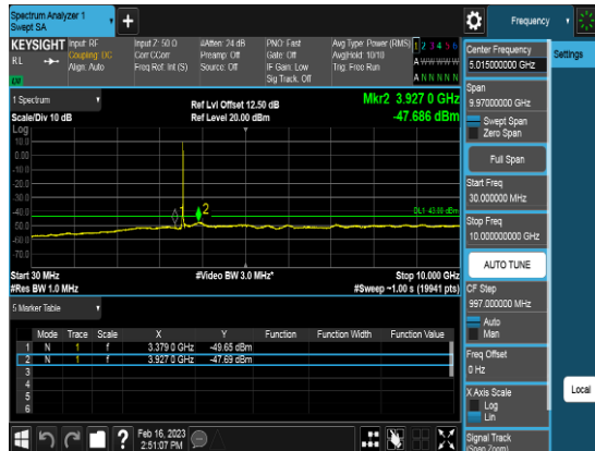
Port1_10M_3555MHz_TM3.1a_CHL_CSE3
