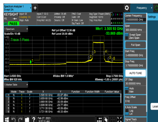
Port2_30M_3684.99MHz_TM3.1_CHH_CSEpart9 6
