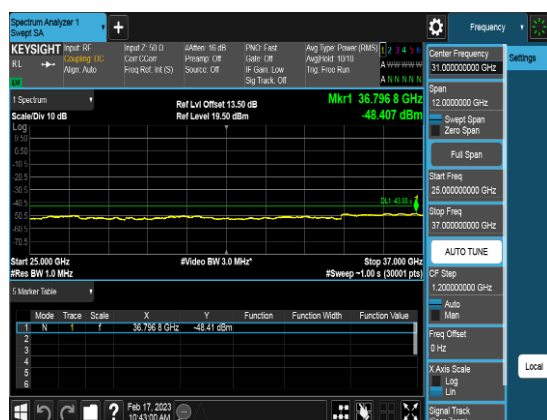
Port1_10M_3624.99MHz_TM3.1a_CHM_CSE3
