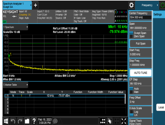
Port1_10M_3555MHz_TM3.1a_CHL_CSE1
