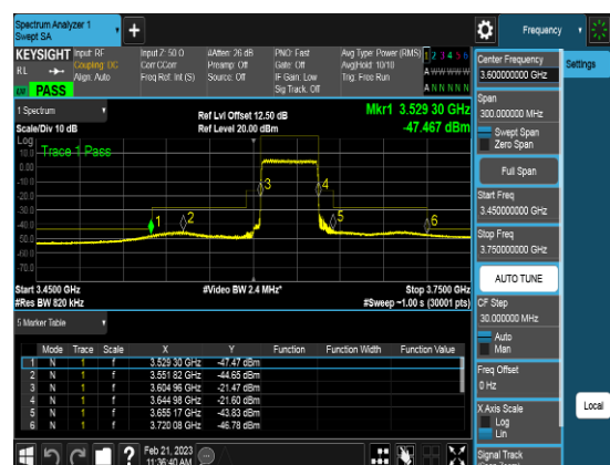
Port2_40M_3624.99MHz_TM3.1_CHM_CSEpart 96
