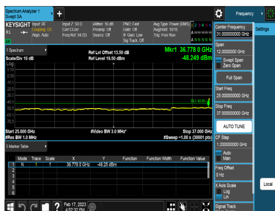
Port2_20M_3560.01MHz_TM3.1_CHL_CSE3
