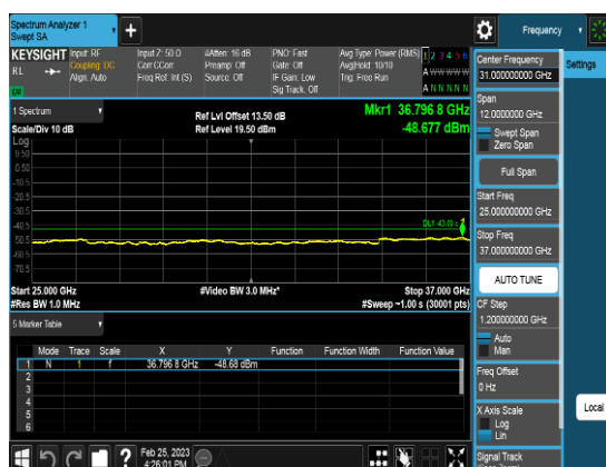
Port2_30M_3624.99MHz_TM3.1_CHM_CSE3
