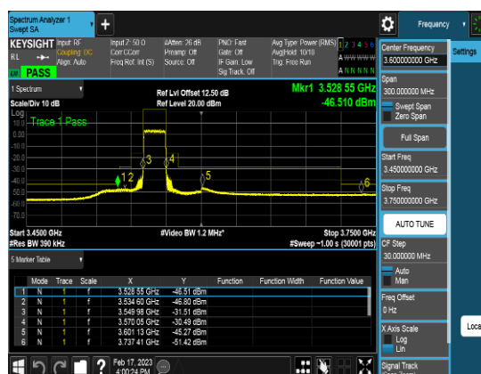
Port2_20M_3560.01MHz_TM3.1_CHL_CSEpart9 6
