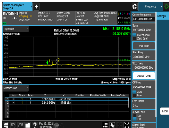
Port2_10M_3624.99MHz_TM3.1_CHM_CSE3
