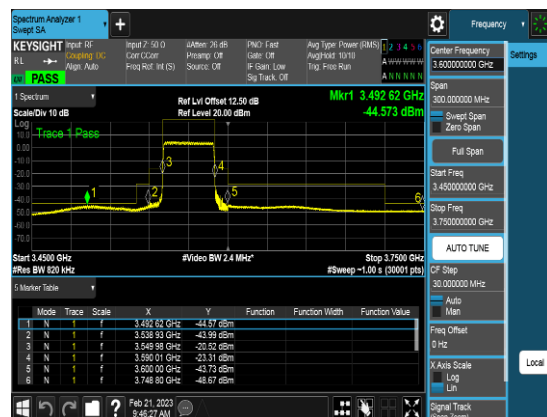
Port2_40M_3570MHz_TM3.1_CHL_CSEpart96
