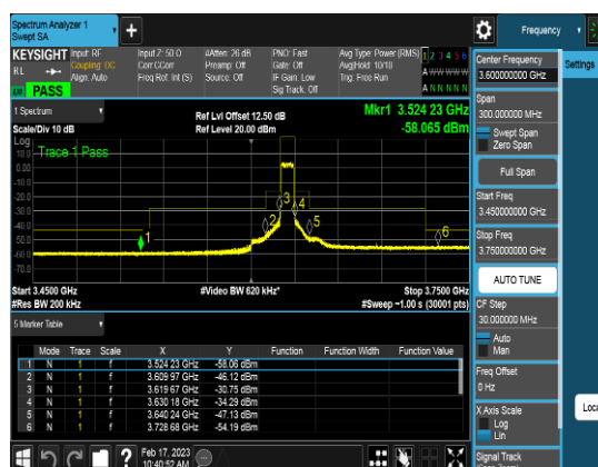
Port1_10M_3624.99MHz_TM3.1a_CHM_CSEpar 196
