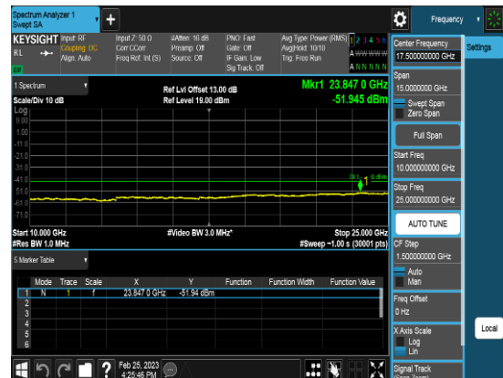
Port2_30M_3624.99MHz_TM3.1_CHM_CSEpart 96
