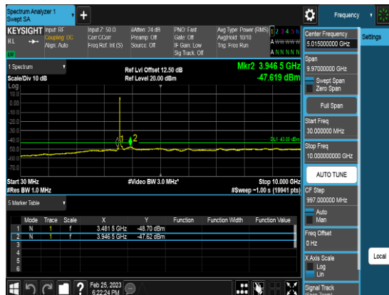
Port2_30M_3565.02MHz_TM3.1_CHL_CSE3
