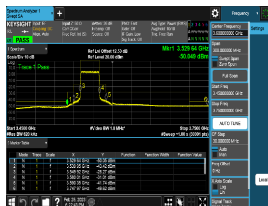
Port2_30M_3565.02MHz_TM3.1_CHL_CSEpart9 6
