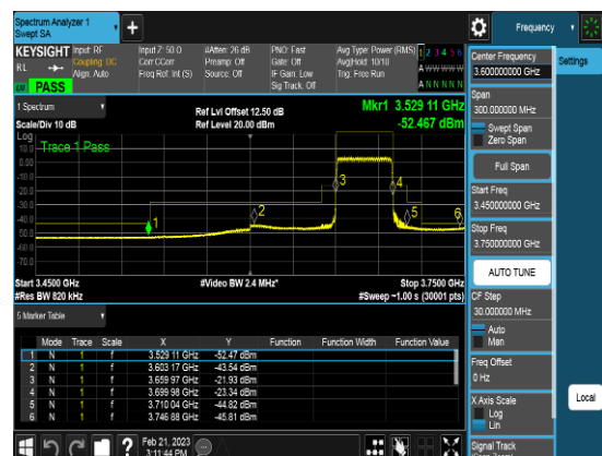
Port2_40M_3679.98MHz_TM3.1_CHH_CSEpart9 6
