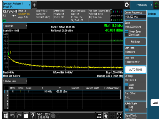
Port2_40M_3679.98MHz_TM3.1_CHH_CSE1
