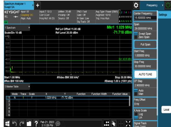
Port2_40M_3679.98MHz_TM3.1_CHH_CSE2
