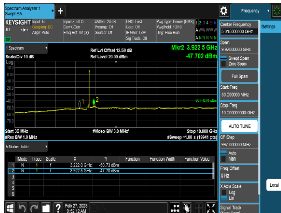
Port2_30M_3684.99MHz_TM3.1_CHH_CSE3
