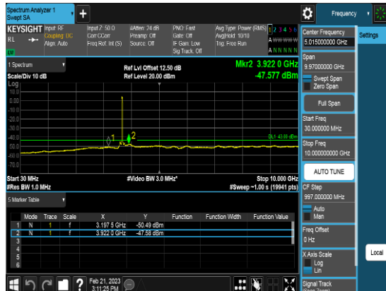
Port2_40M_3679.98MHz_TM3.1_CHH_CSE3
