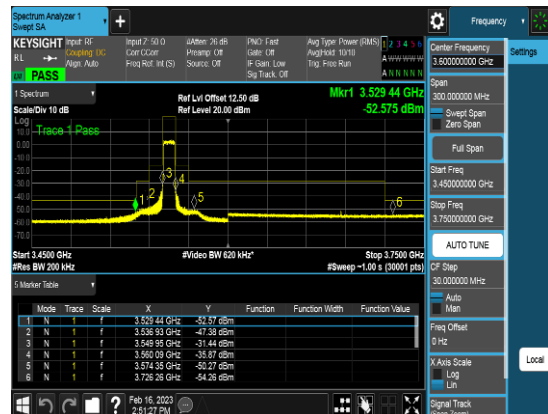
Port1_10M_3555MHz_TM3.1a_CHL_CSEpart96
