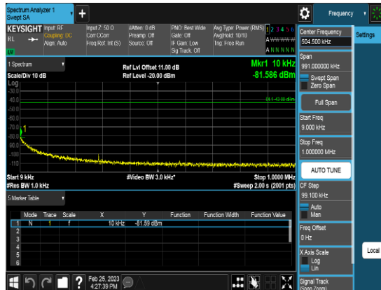
Port2_30M_3624.99MHz_TM3.1_CHM_CSE1
