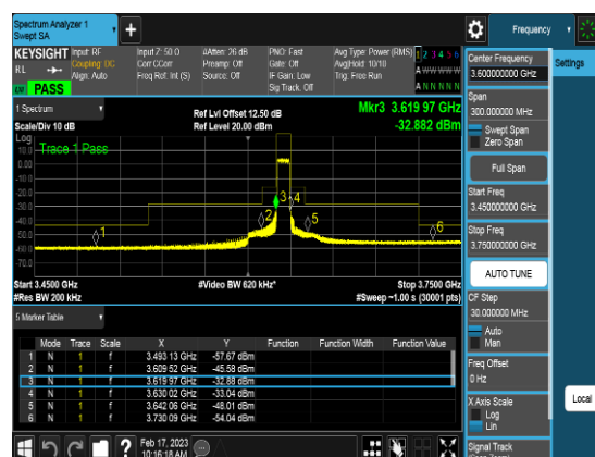
Port2_10M_3624.99MHz_TM3.1_CHM_CSEpart 96
