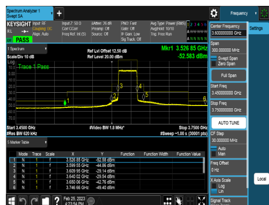
Port2_30M_3624.99MHz_TM3.1_CHM_CSEpart 96
