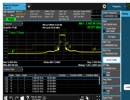
Port2_20M_3624.99MHz_TM3.1_CHM_CSEpart 96
