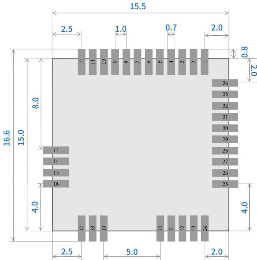
Figure 4: RAK11720 Layout
