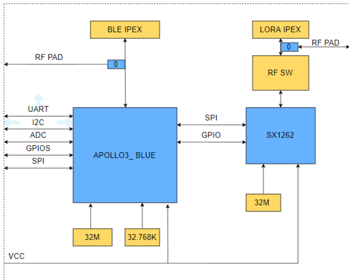
Figure 1: RAK11720 System Block Diagram
