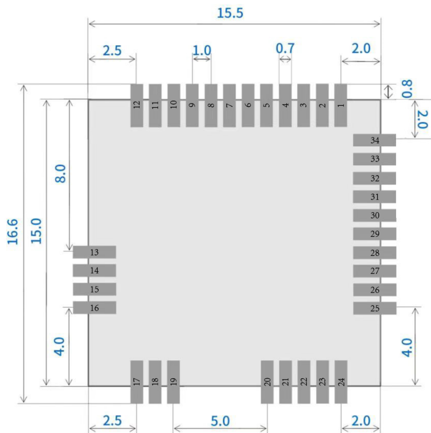
Figure 4: RAK11720 Layout
