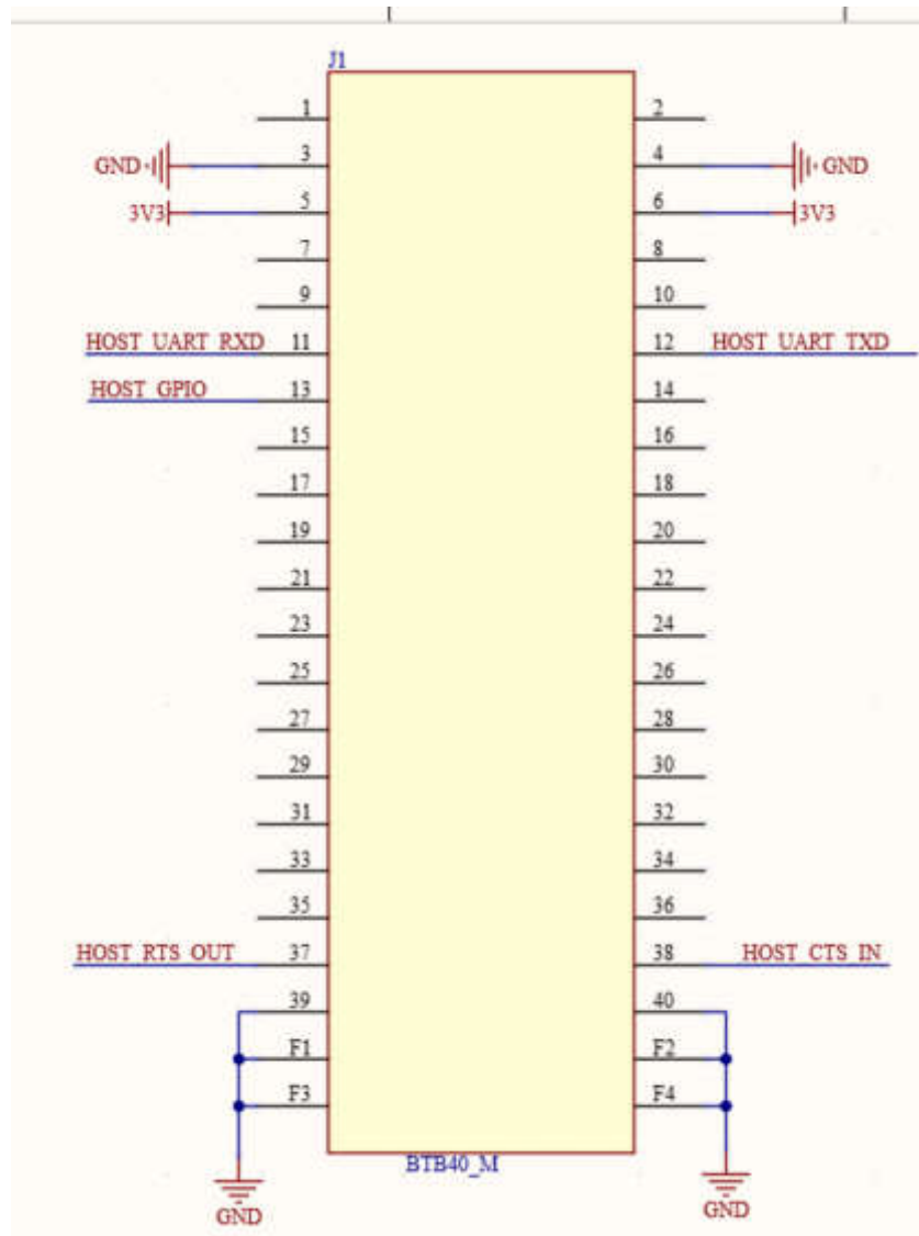
Figure 5: RAK13401 Connector Connection
