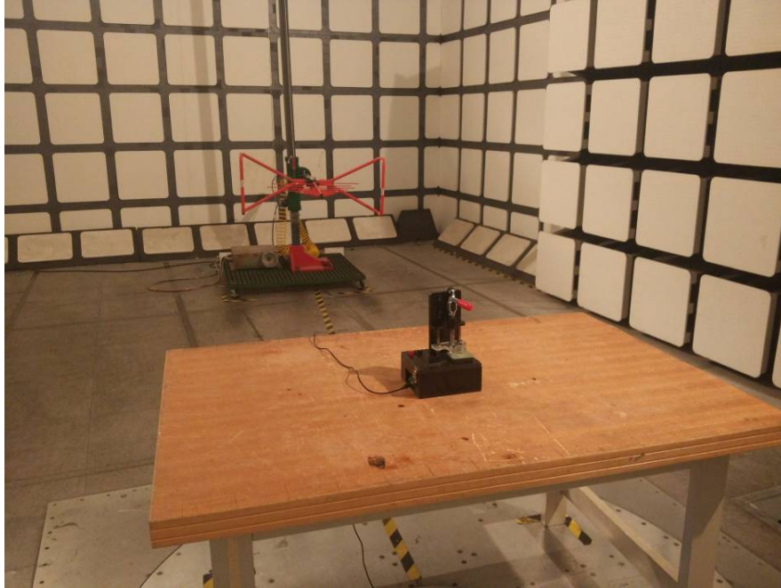
Radiated Emissions View – Onboard Antenna (Below 1 GHz)
