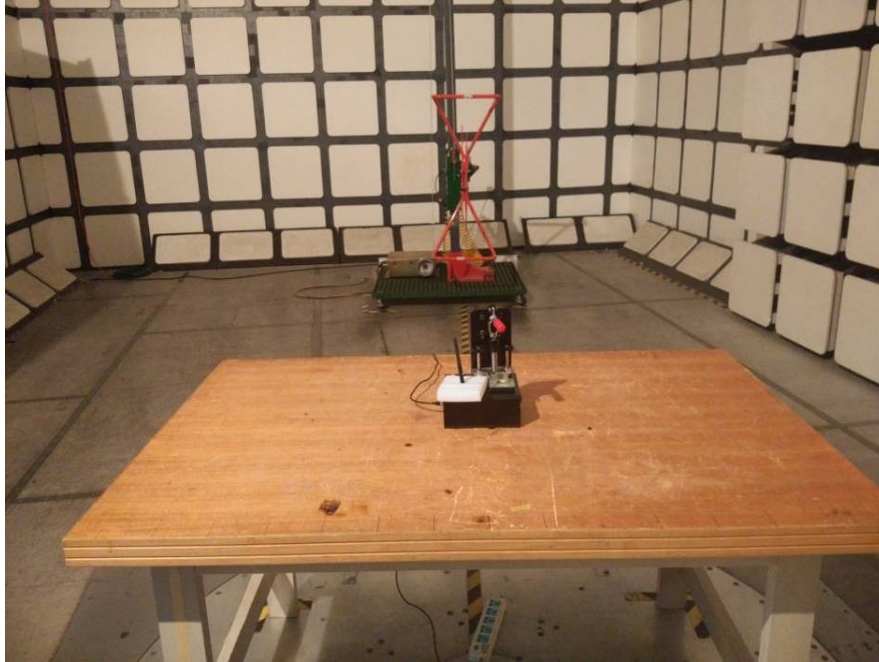
Radiated Emissions View – External Antenna (Below 1 GHz)
