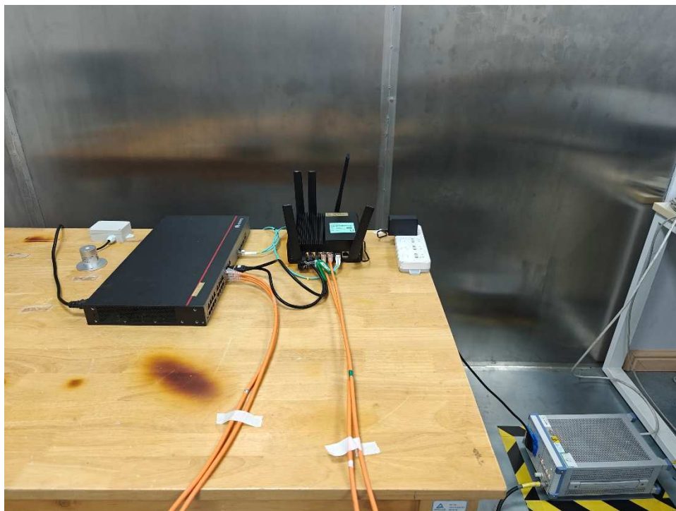
Photograph 3: Set-up for Conducted Emissions, AC Mains
