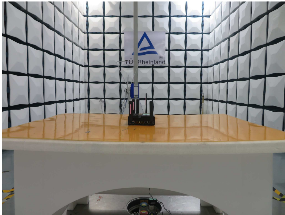
Photograph 1: Set-up for Radiated Spurious Emissions, below 1GHz
