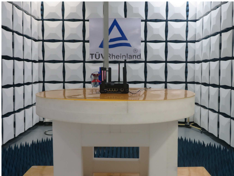
Photograph 2: Set-up for Radiated Spurious Emissions, above 1GHz
