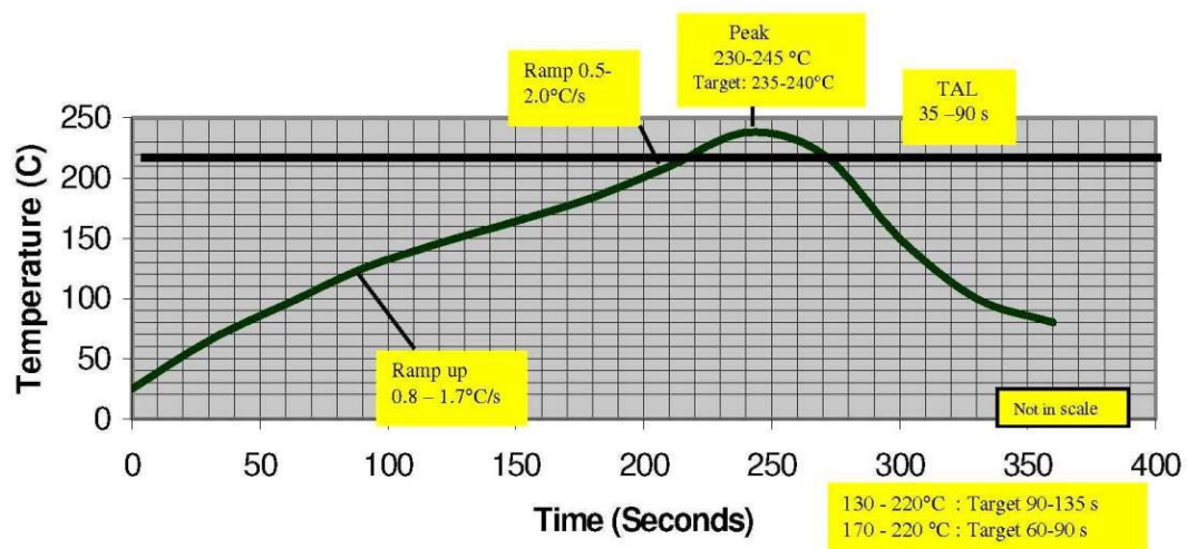
Figure 3-10 Temperature Graph
