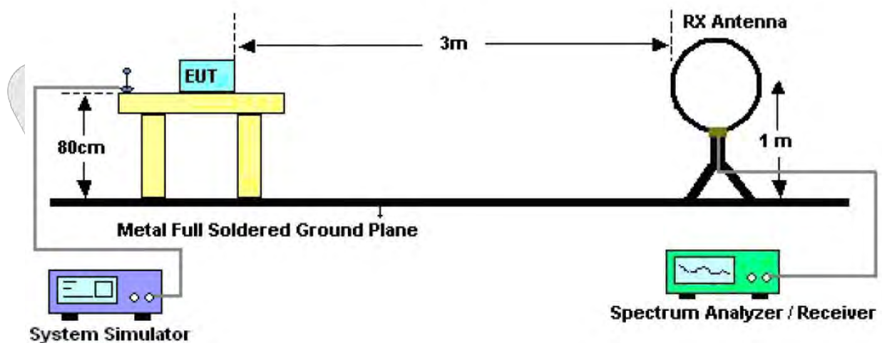
Figure 1. Below 30MHz
