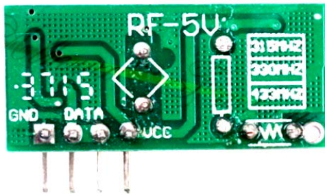
BACK VIEW OF SUB-BOARD OF 433 MHZ RECEIVER
