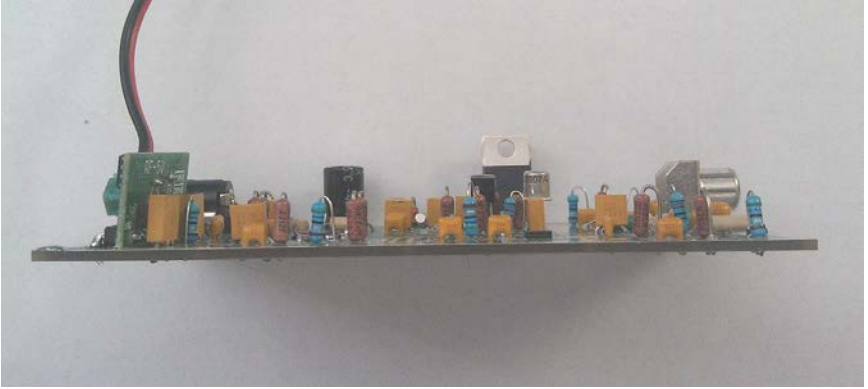
LEFT SIDE VIEW OF PWB ASSEMBLY
