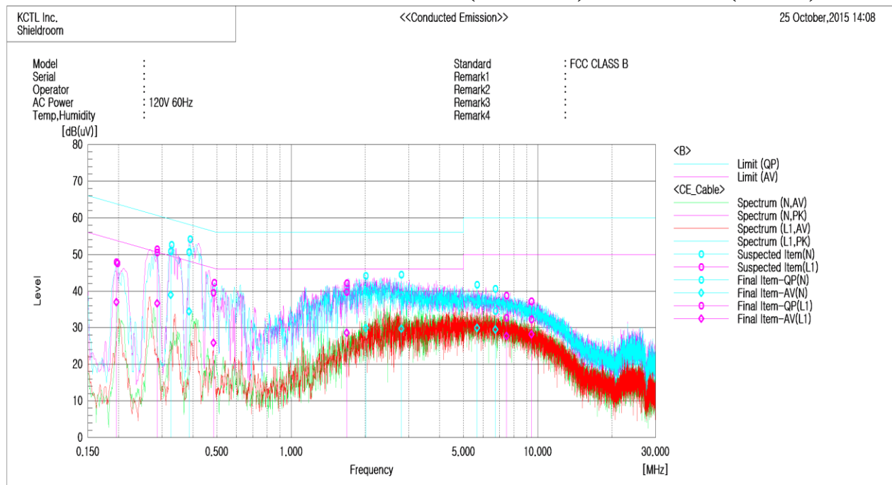
Figure 4. plot of Conducted Emission
