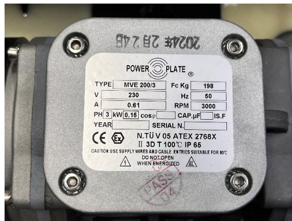
Motor: MVE200/3
