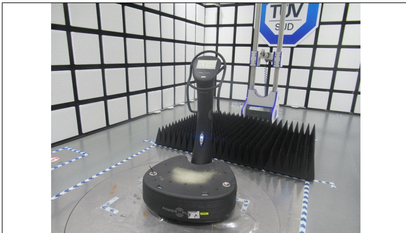
Radiated Emission test (18000 to 40000MHz)
