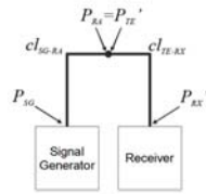
FIGURE 4-3 CABLE REFERENCE CALIBRATION CONFIGURATION
