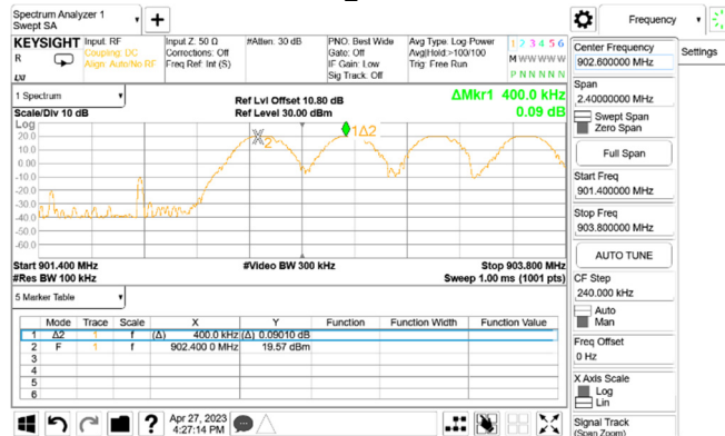
FSK_CH32CH33
