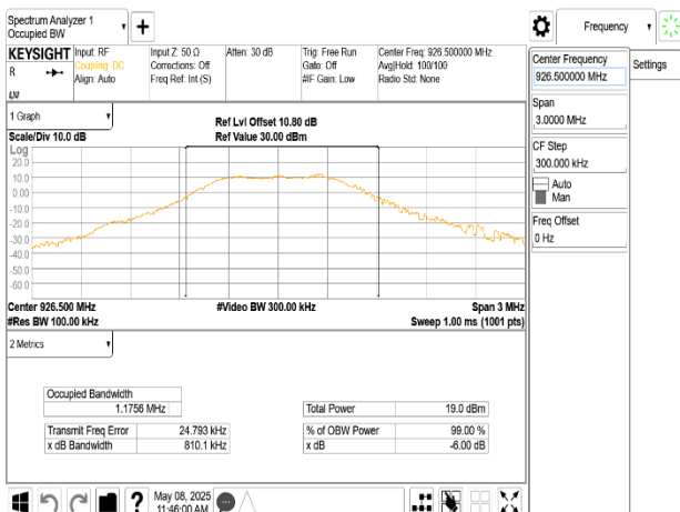
OBW_OFDM 1M_HighCH-926.5MHz
