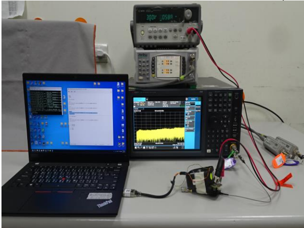
FCC_P15_247+IC_RSS_247_WLAN_2.4G_Conducted_Setup
