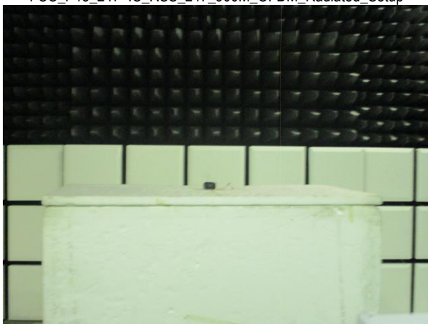
FCC_P15_247+IC_RSS_247_900M_OFDM Radiated_Setup
