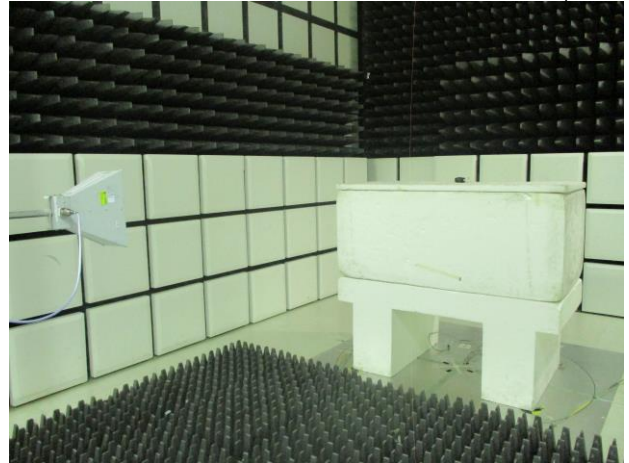
FCC_P15_247+IC_RSS_247_900M_FSK_Radiated_Setup
