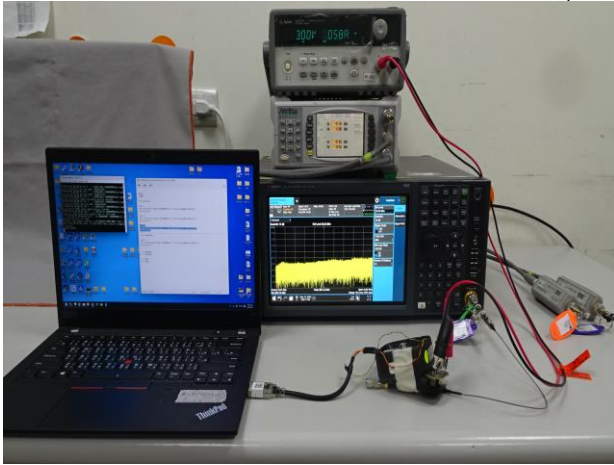
FCC_P15_247+IC_RSS_247_900M_OFDM_Conducted_Setup
