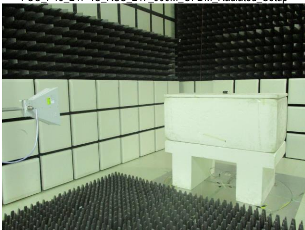
FCC_P15_247+IC_RSS_247_900M_OFDM Radiated_Setup
