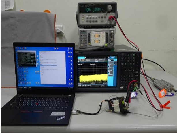
FCC_P15_247+IC_RSS_247_WLAN_2.4G_Conducted_Setup
