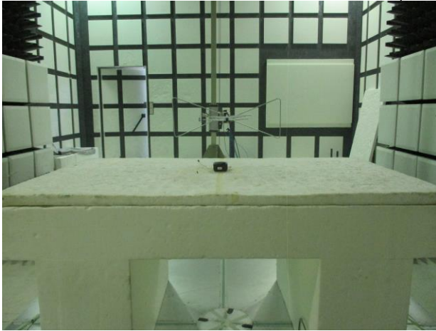
FCC_P15_247+IC_RSS_247_WLAN 2.4G_Radiated_Setup
