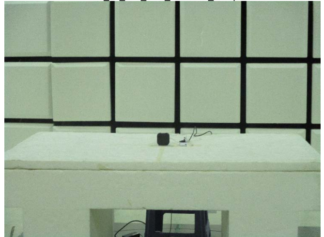
Part 15 247 FSK Radiated Setup
