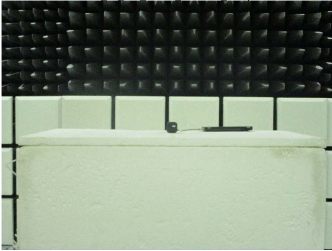
Part 15 247 OFDM Radiated Setup
