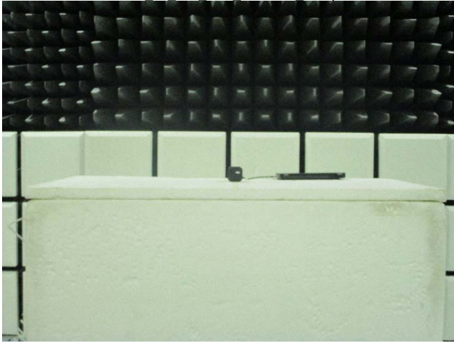
Part 15 247 FSK Radiated Setup
