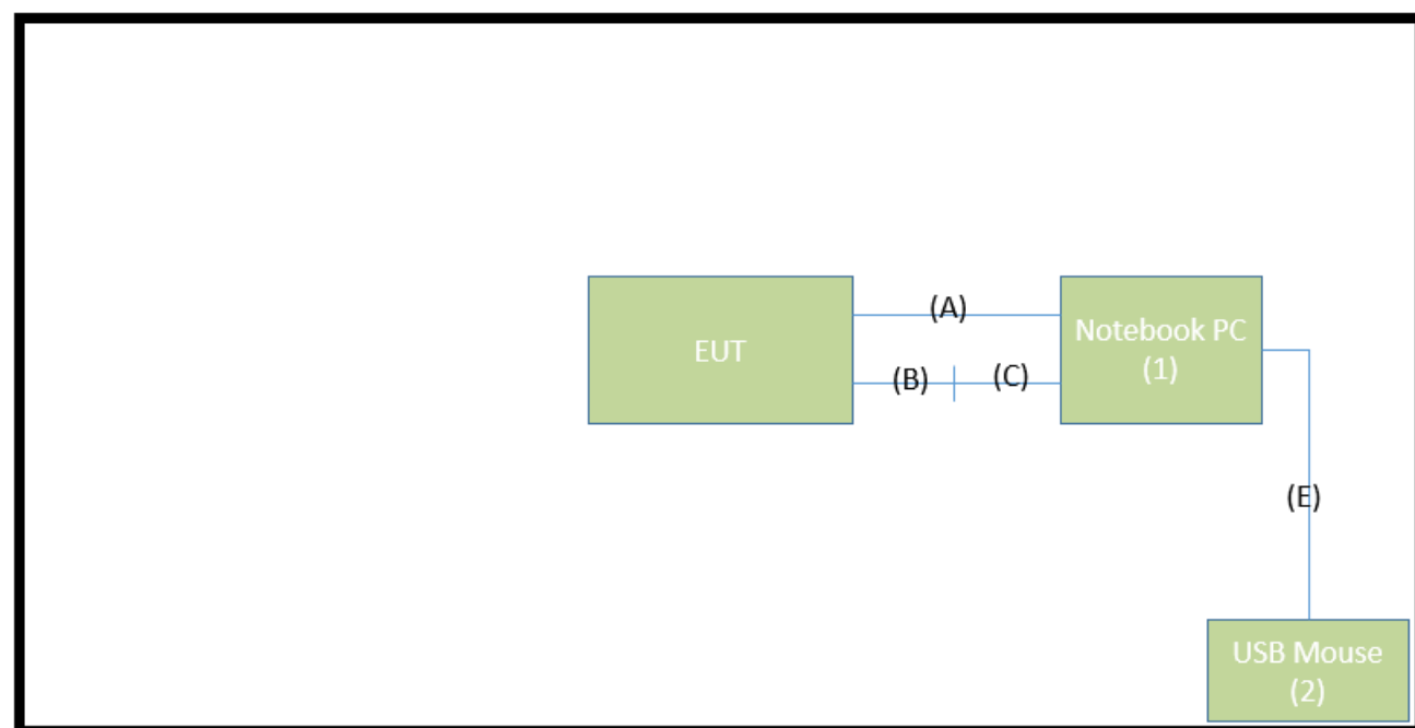
Connection Diagram
