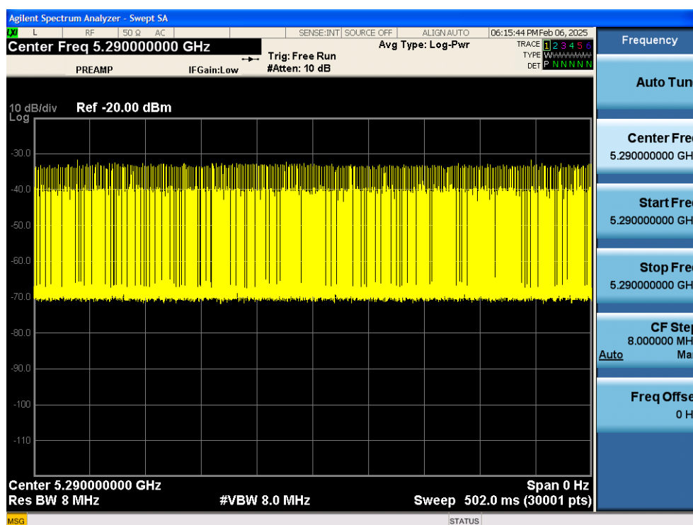
Channel Loading Plot - 802.11ax80-5290MHz
