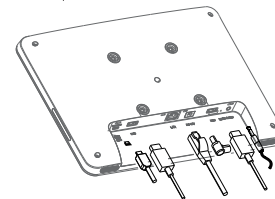
Cables connection
