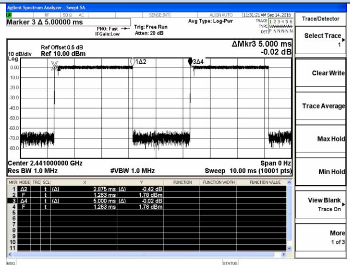
2DH5-2441MHz
