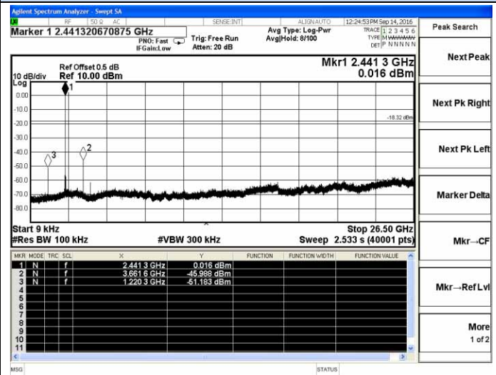
2DH1-Middle channel
