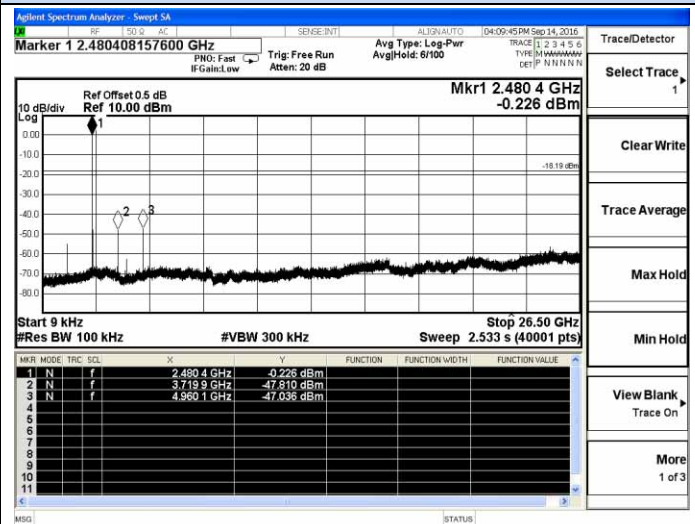
3DH1-High channel
