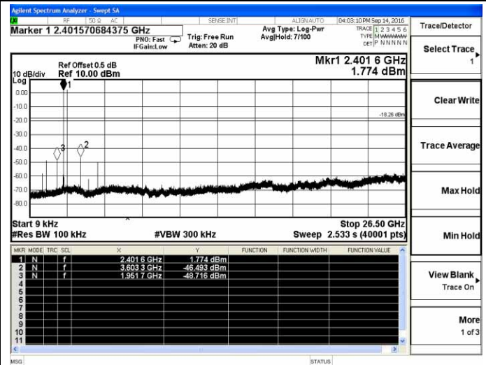
3DH1-Low channel
