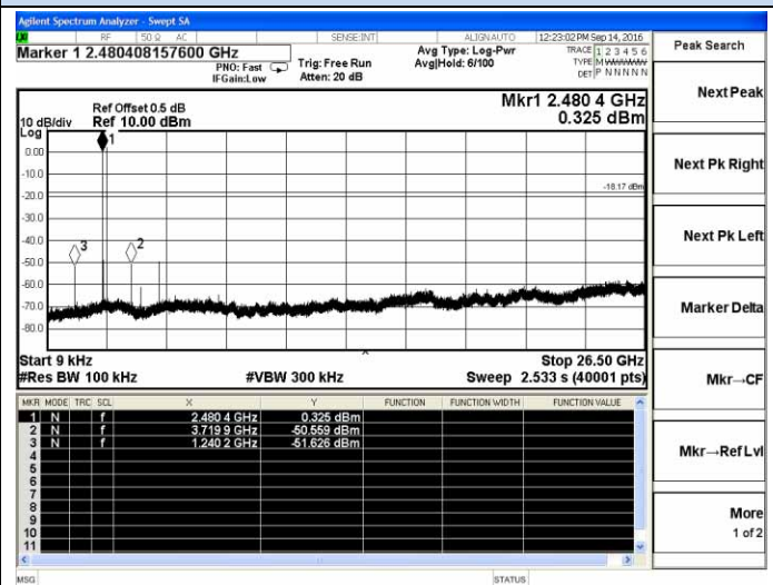
2DH1-High channel
