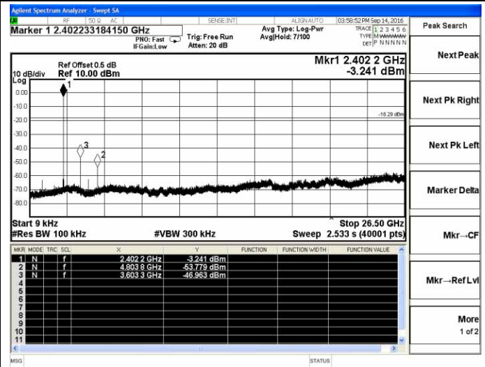
2DH1-Low channel
