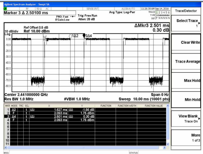
2DH3-2441MHz
