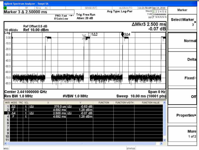
2DH1-2441MHz
