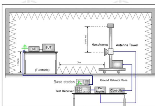
Figure 2. above 1GHz
