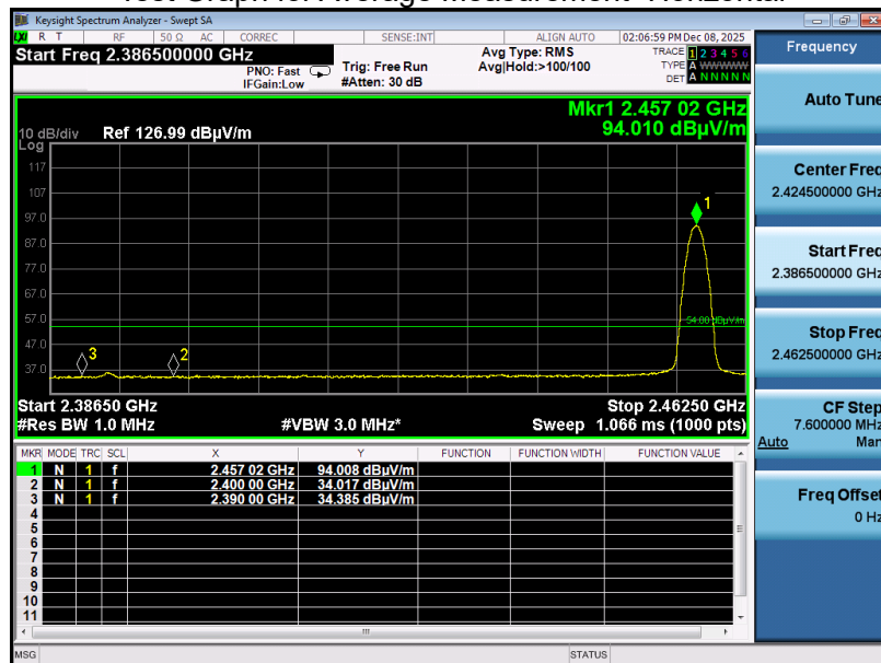
Test Graph for Average Measurement- Horizontal
