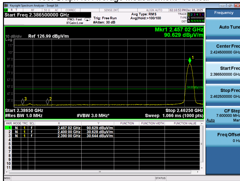
Test Graph for Average Measurement- Vertical
