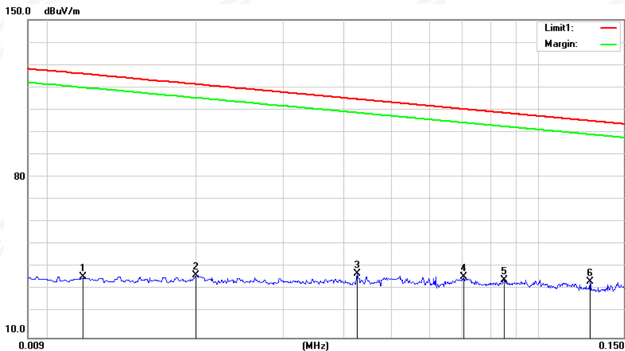
RSE-9KHz-150KHz
