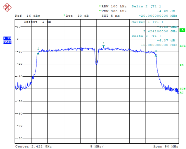
CH3 / 2422 MHz
