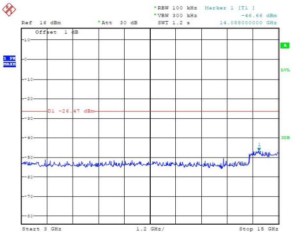
3G Hz~15GHz
