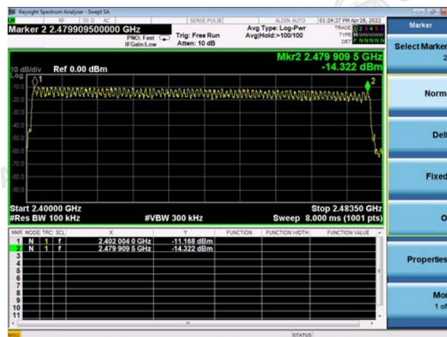
8-DPSK Modulation
