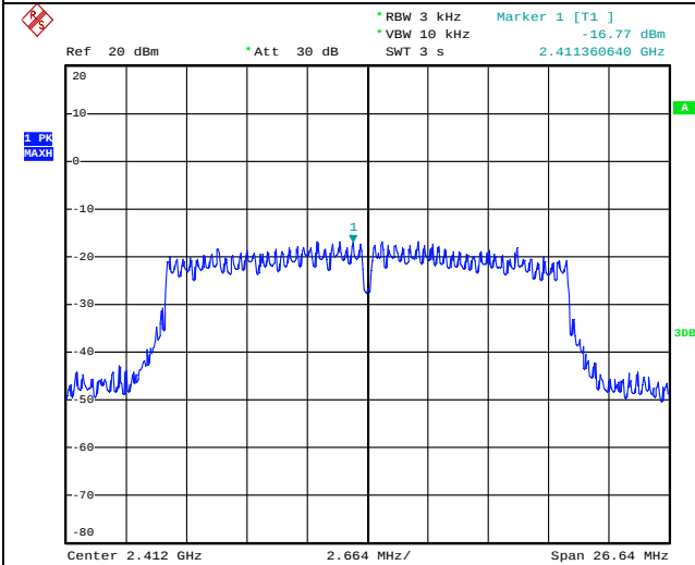
2412 MHz
